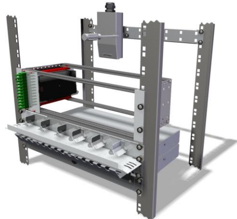
View of cable tube divider installed on distribution frame
