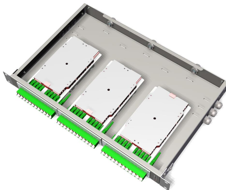
View of 1U modular patch panel equipped with 3 PS-01 modules and 9 cable glands.
