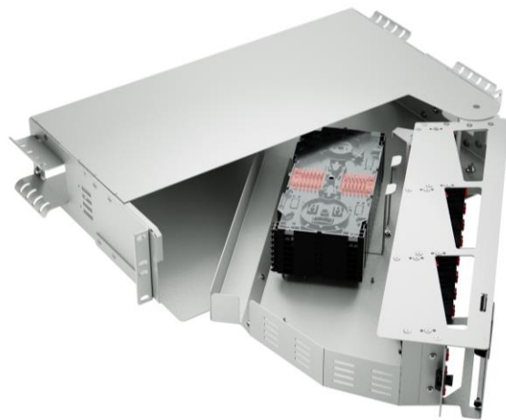
View of 2U patch panel
