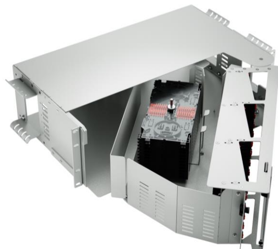
View of 3U patch panel
